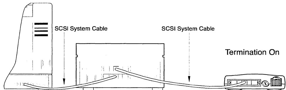
Connecting Pocket SCSI/Link as the Last Device
