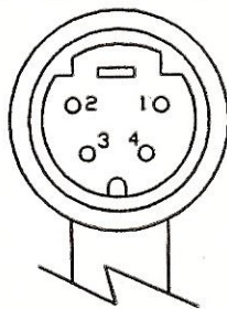
Figure 16 - ADB connector male cable face
