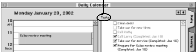
Daily Calendar
