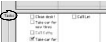
Weekly Calendar
