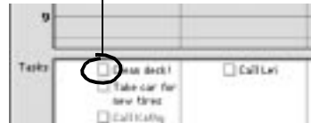
Weekly Calendar
