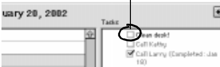
Daily Calendar
