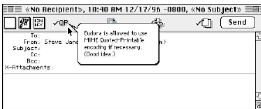
Balloon Help
