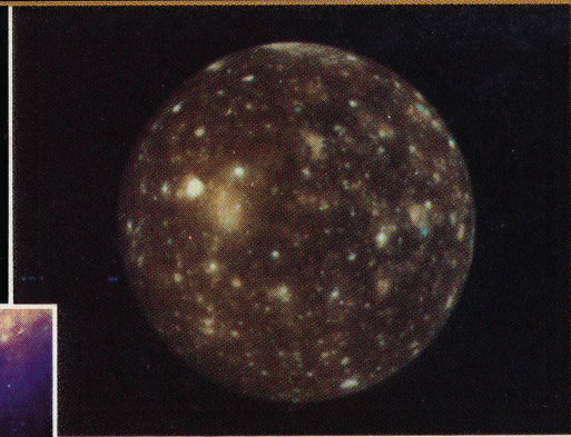
Callisto, one of Jupiter's moons
