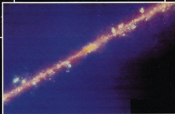
Central Milky Way (Infra Red)
