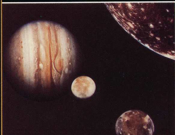
Jupiter and moons
