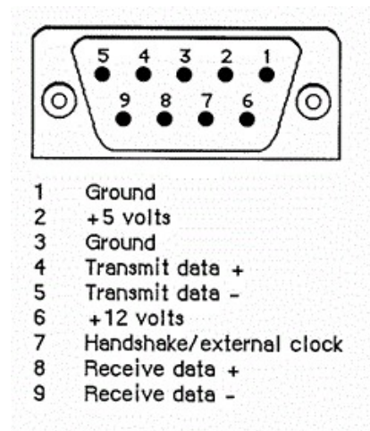
Figure 3. Pinout for SCC Output Jacks
